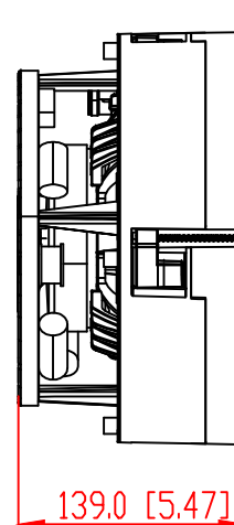
MOUNTING DEPTH
